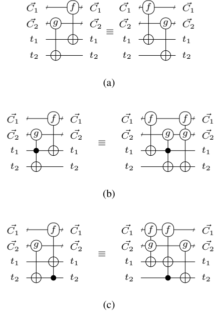
Fig. 4: Rewriting rules
