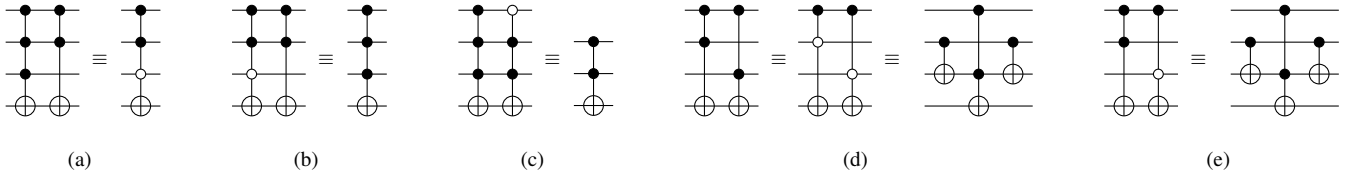
Fig. 6: Applied reductions
