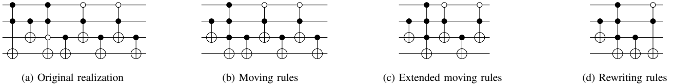
Fig. 5: Circuit optimization wrt. different moving rules
